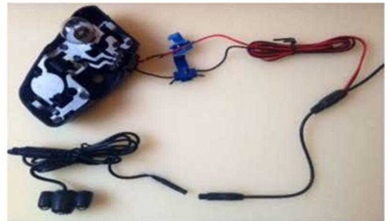
Reversing camera connection to reversing bulb.
