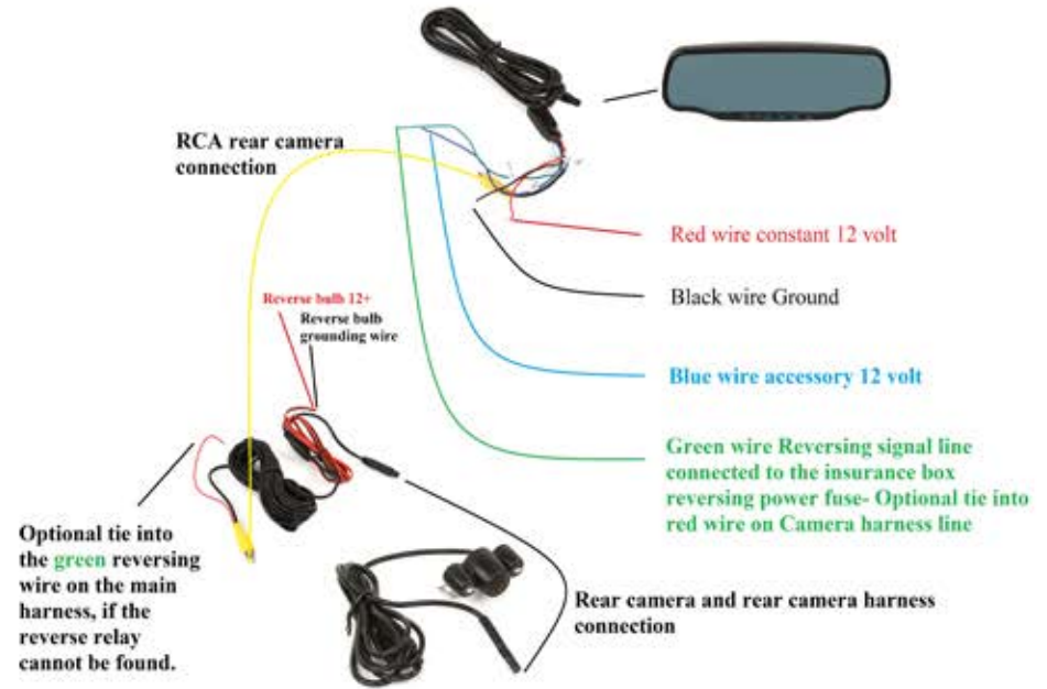
Overview of wiring diagram.
